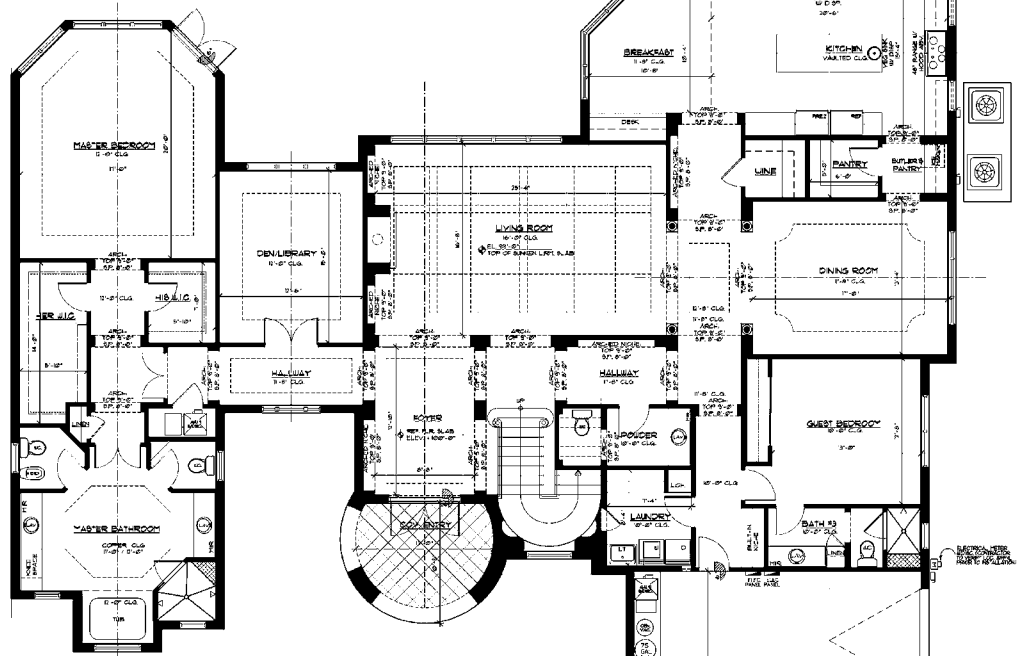
First Floor Elevation
